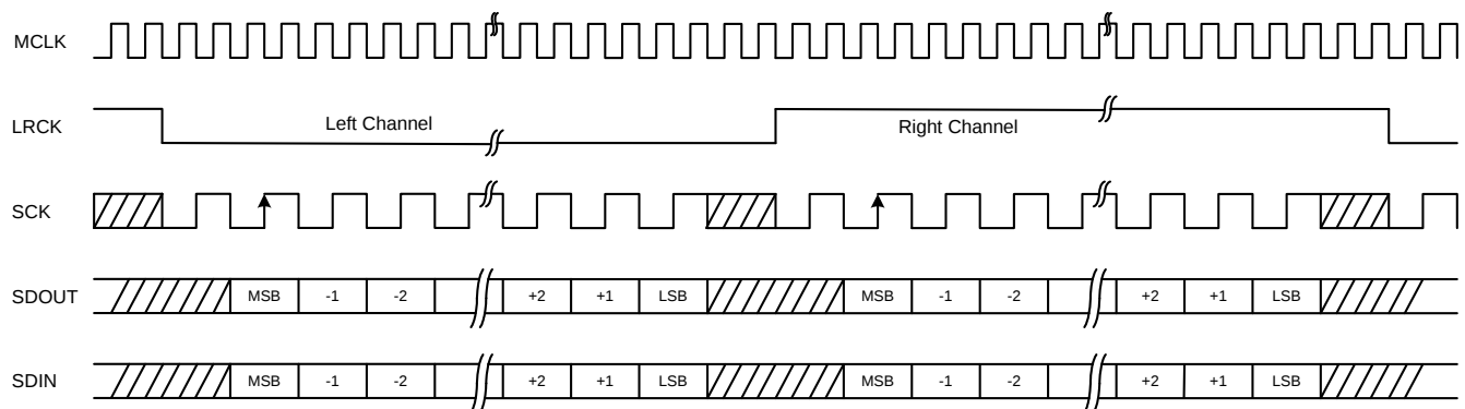
Figure 8. I2S Format
