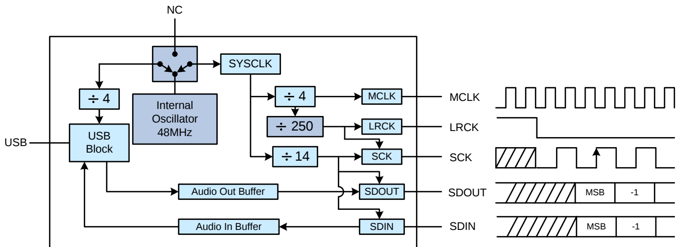
Figure 11. Configuration 1 Example
